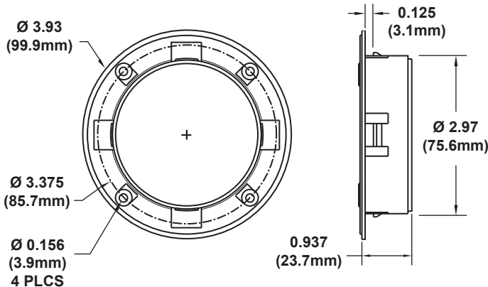
4" MIRAGE MOUNTING RETAINER
