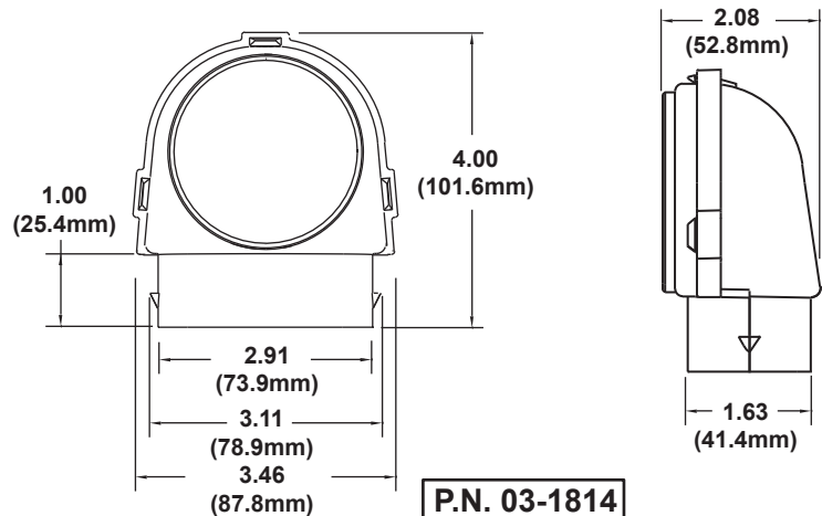
2-1/2" 90 DEGREE LOUVER ADAPTER
