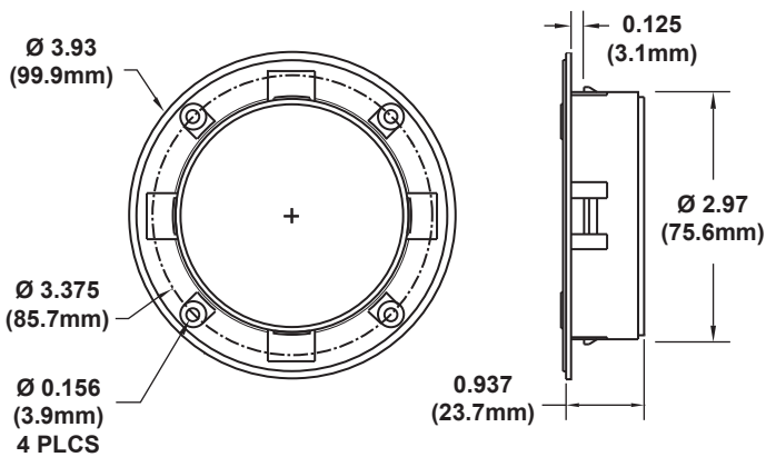
4" TRADITIONAL FRONT PANEL W/ VANES
