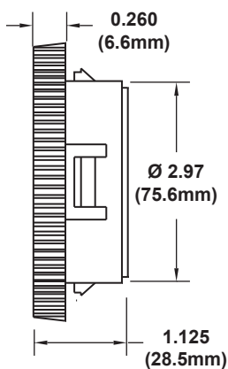
4" MIRAGE SNAP-IN LOUVER w/o HOSE ADAPTER
