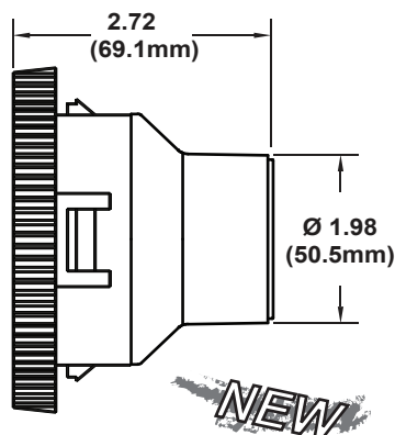
4" MIRAGE SNAP-IN LOUVER w/ 2" HOSE ADAPTER
