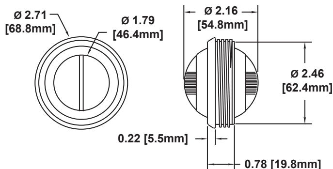
CANYON BALL & RETAINER
