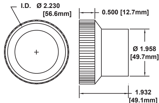
MOUNTING BEZEL
