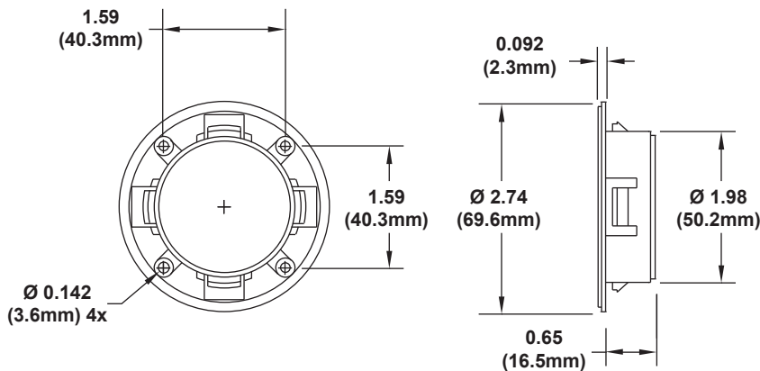
2" MIRAGE RETAINER
