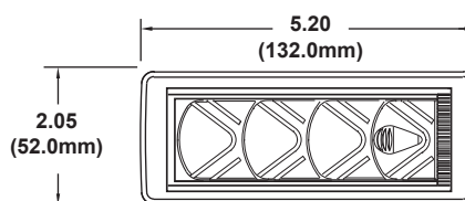
NARROW FRAME VERSION WITHOUT HOLES P.N. 06-2020-3
