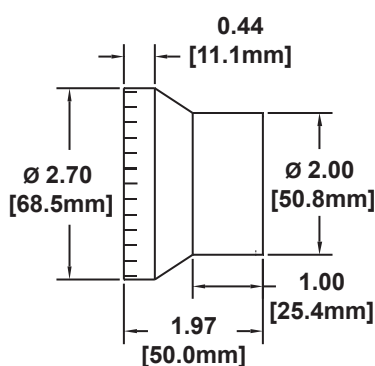
CANYON BALL & RETAINER
