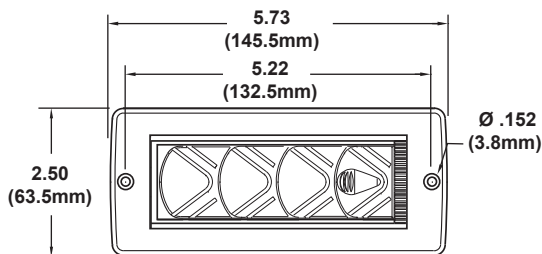
WIDE FRAME VERSION WITH HOLES P.N. 06-2020
