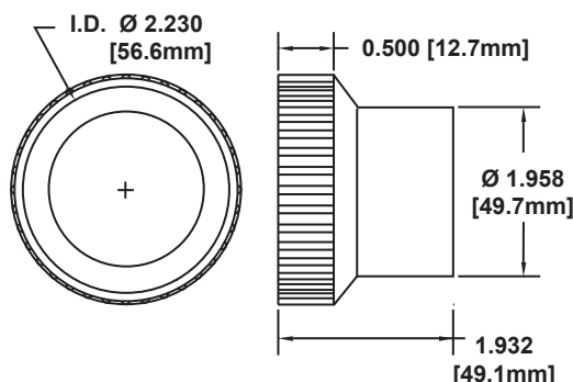
STARLIGHT MOUNTING BEZEL
