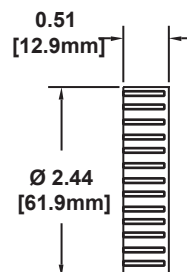
STARLIGHT MOUNTING BEZEL
