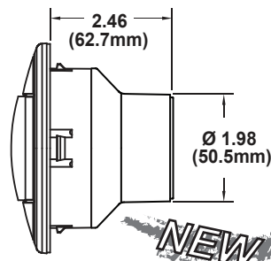
4" SIERRA SNAP-IN LOUVER w/ 2" HOSE ADAPTER
