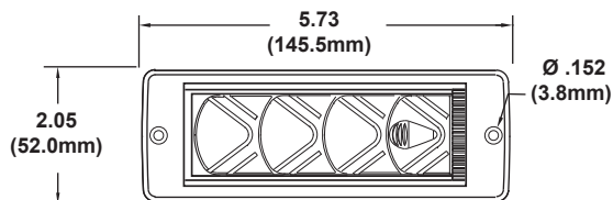
NARROW FRAME VERSION WITH HOLES P.N. 06-2020-2
