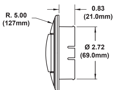
4" SIERRA FRONT PANEL w/ VANES
