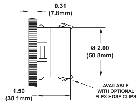
2" MIRAGE SNAP-IN LOUVER w/ 2" HOSE ADAPTER (WITH CLIPS P.N.06-2000-1-CL)
