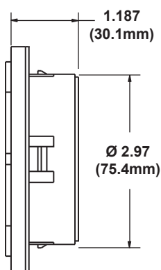
4" TRADITIONAL MOUNTING RETAINER
