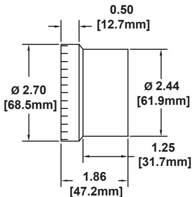
CANYON BALL & RETAINER
