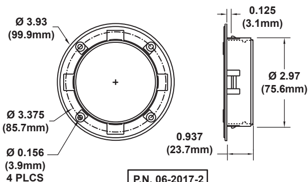
4" SIERRA MOUNTING RETAINER
