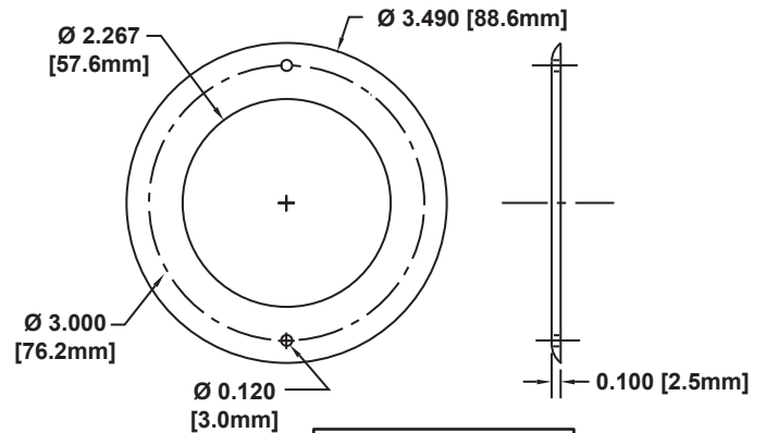
MOUNTING BEZEL
