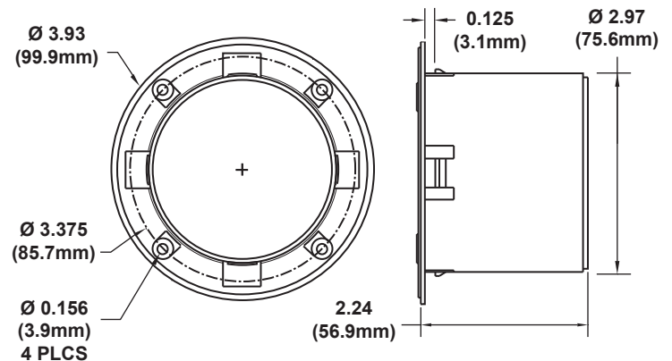
4" MTG RETAINER w/ STANDARD 3 INCH HOSE ADAPTER
