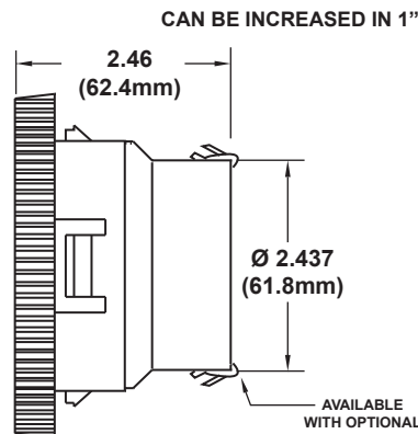
4" MIRAGE SNAP-IN LOUVER w/ 2-1/2" HOSE ADAPTER
