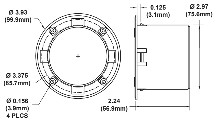
4" MTG RETAINER W/ STANDARD 3 INCH HOSE ADAPTER ASSEMBLED P/N 06-2016-4-L
