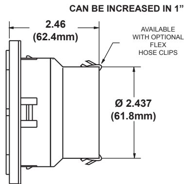
4" MTG RETAINER W/ STANDARD 3 INCH HOSE ADAPTER ASSEMBLED P/N 06-2016-4-L
