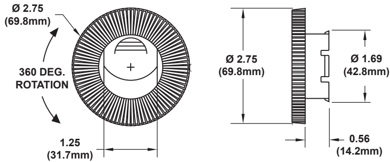
2" MIRAGE FRONT PANEL w/VANES
