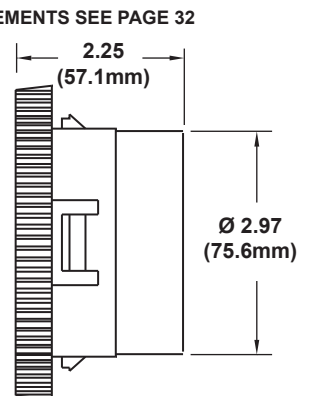
4" MIRAGE SNAP-IN LOUVER w/ 3" HOSE ADAPTER (OPTIONAL SHORTER LENGTH)
