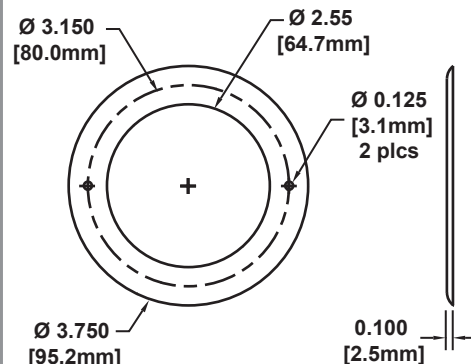
MOUNTING BEZEL
