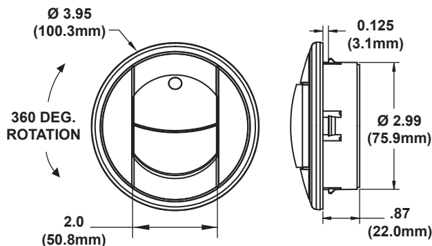
4" SIERRA SNAP-IN LOUVER w/o HOSE ADAPTER
