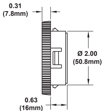
2" MIRAGE SNAP-IN LOUVER w/o HOSE ADAPTER
