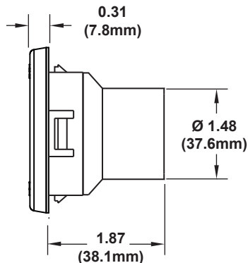
2" SONORA RETAINER
