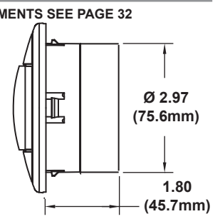
4" SIERRA SNAP-IN LOUVER w/ 3" HOSE ADAPTER (OPTIONAL SHORTER LENGTH)
