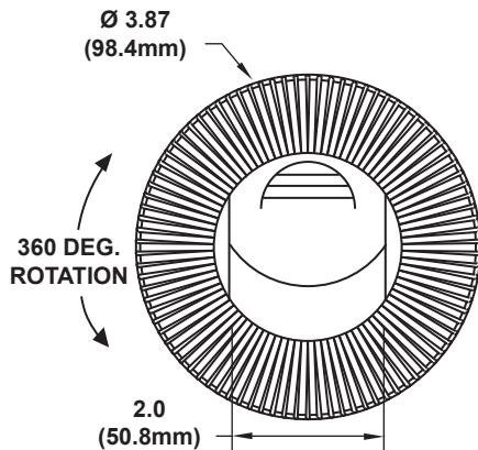
4" MIRAGE FRONT PANEL w/ VANES
