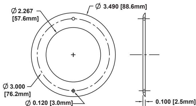
STARLIGHT MOUNTING BEZEL
