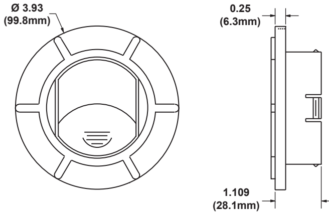
4" TRADITIONAL FRONT PANEL W/ VANES
