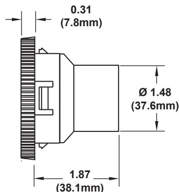
2" MIRAGE RETAINER
