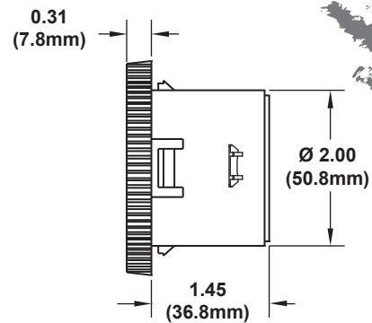
2" MIRAGE SNAP-IN LOUVER w/2" HOSE ADAPTER w/BARBS
