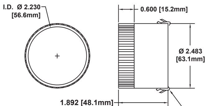
STARLIGHT BALL & RETAINER
