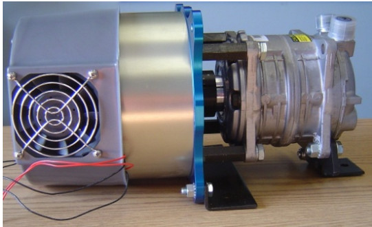
DC electric motor, direct drive with TM-08 compressor & CMG-0.67-13 sealed motor
